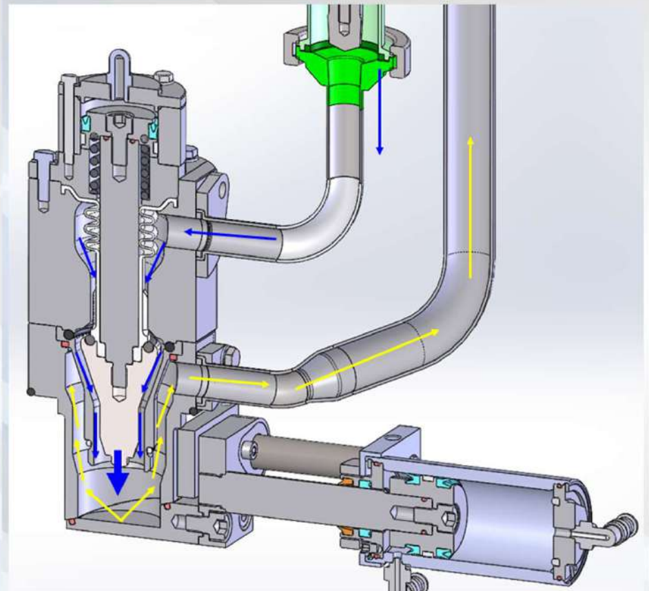
CIP cycle
