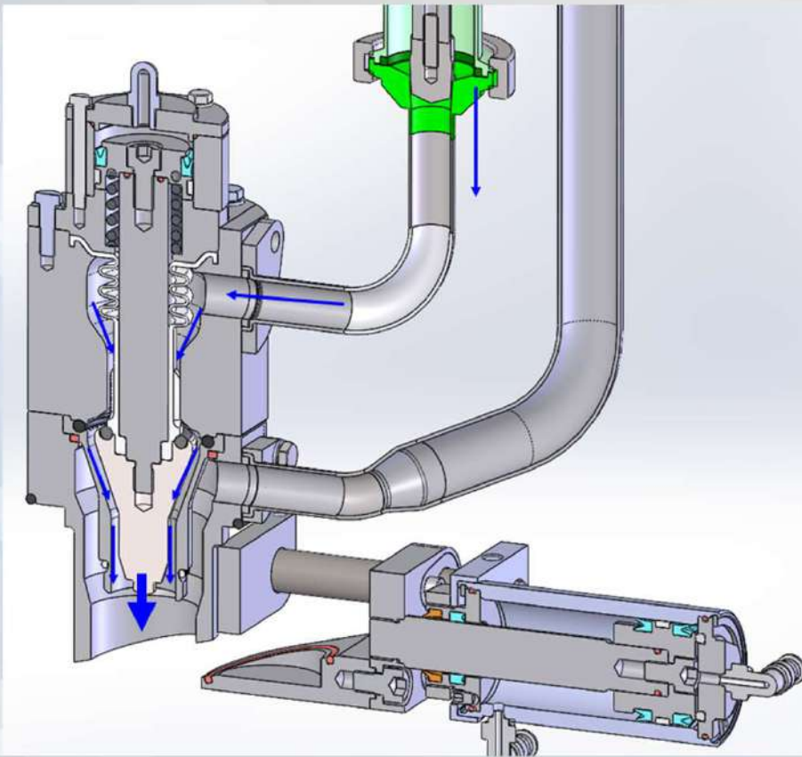
Filling cycle
